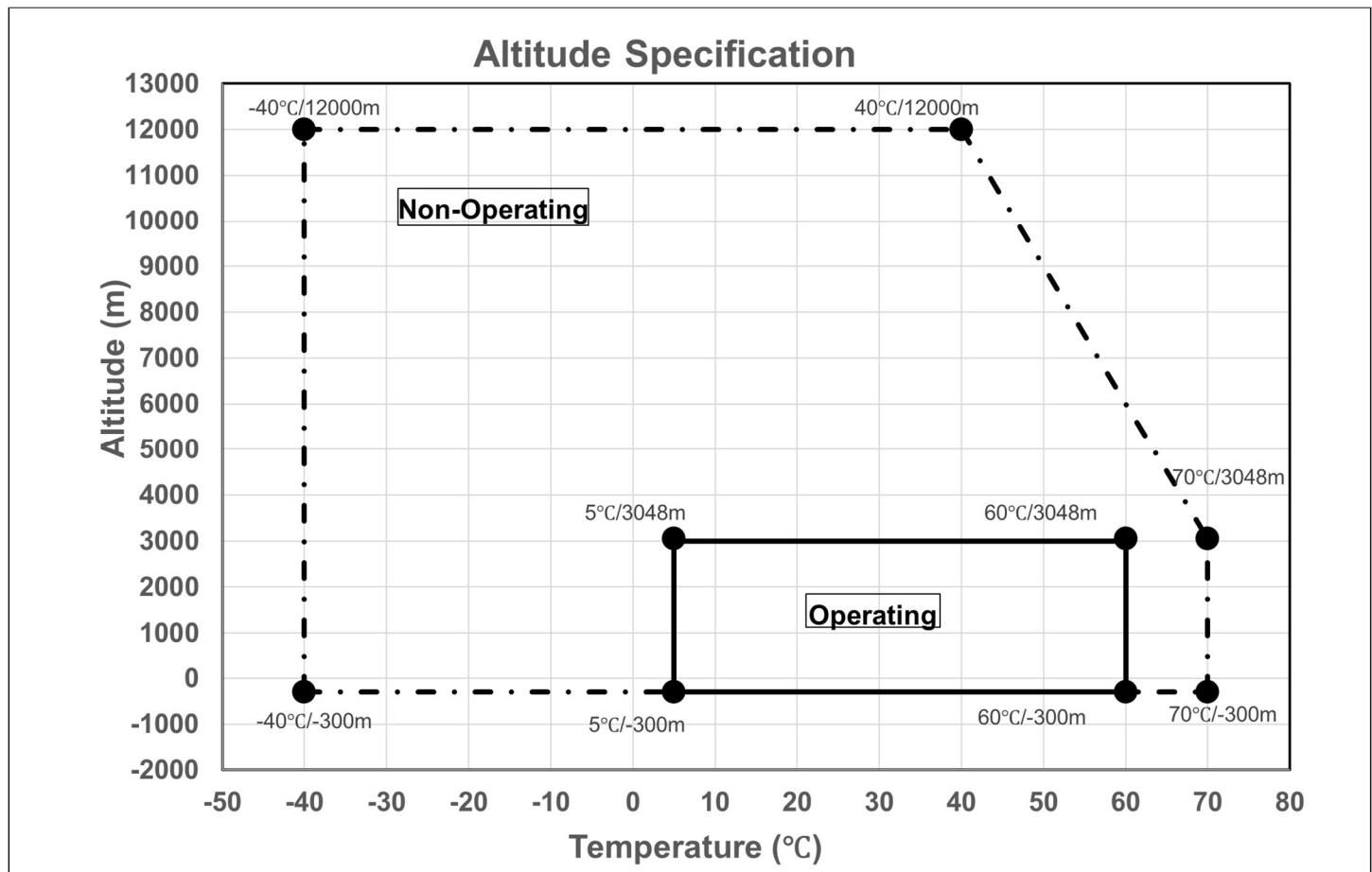
Figure 4 Limits of temperature and altitude
