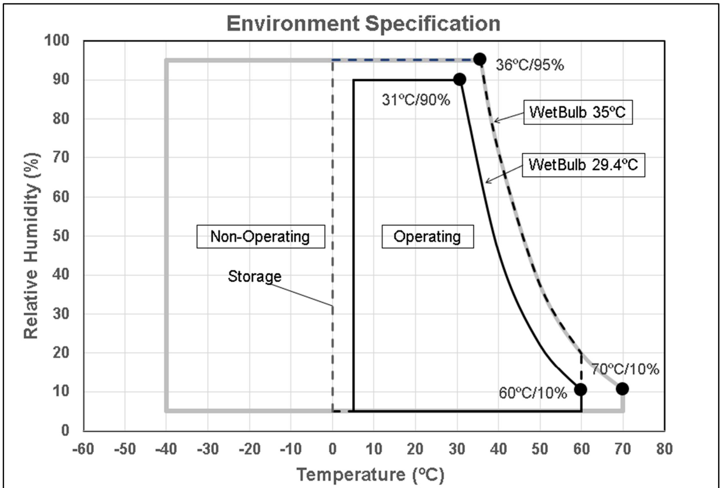
Figure 5 Limits of temperature and humidity.
