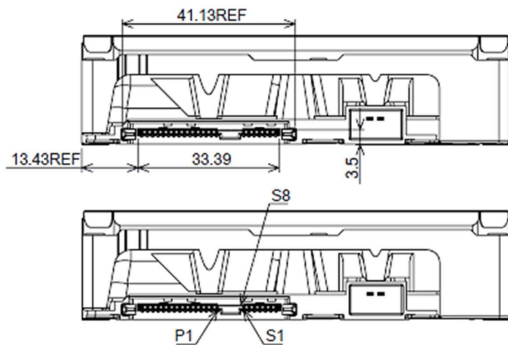
Figure 9 Connector locations
